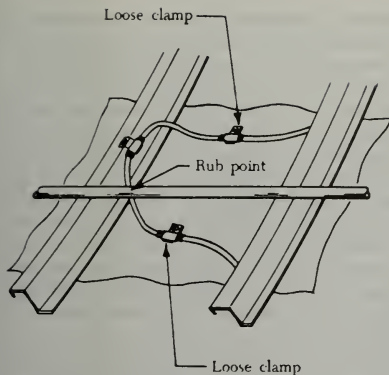
FIGURE 9-19. Rubbing interference.
